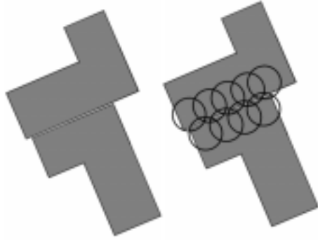
(a) This might be considered a single collision between two faces (b) An increasing number of sphere collisions will be detected at each level of detail
